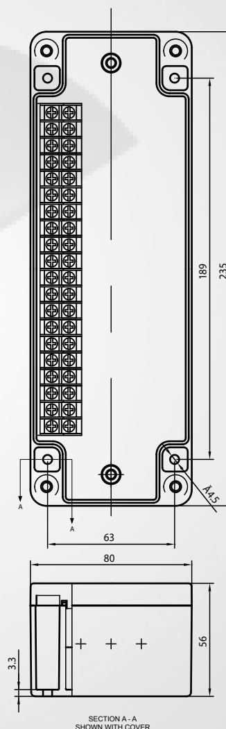
SECTION A - A SHOWN WITH COVER
