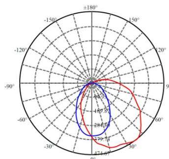
7W Light Distribution Curve →
