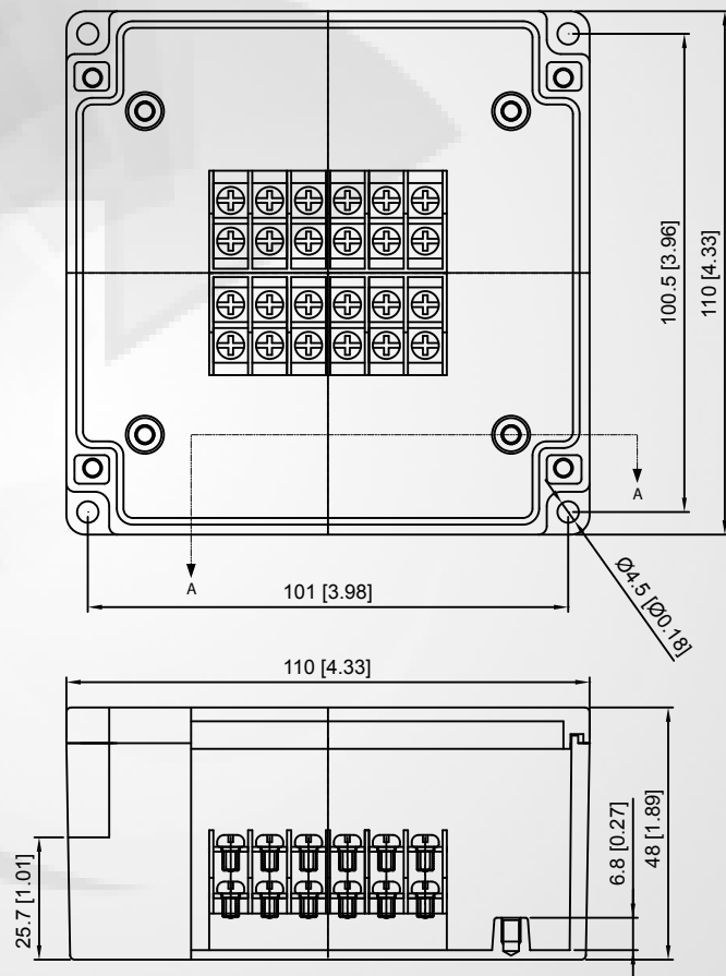
SECTION A - A SHOWN WITH COVER
