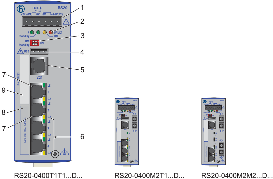
Figure 1: Device variants with 4 × 10/100 Mbit/s ports (RS20-0400...)
