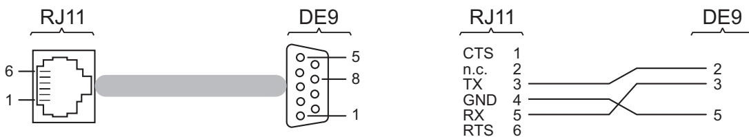
Figure 15: Pin assignment of the V.24 interface and the DE9 connector
