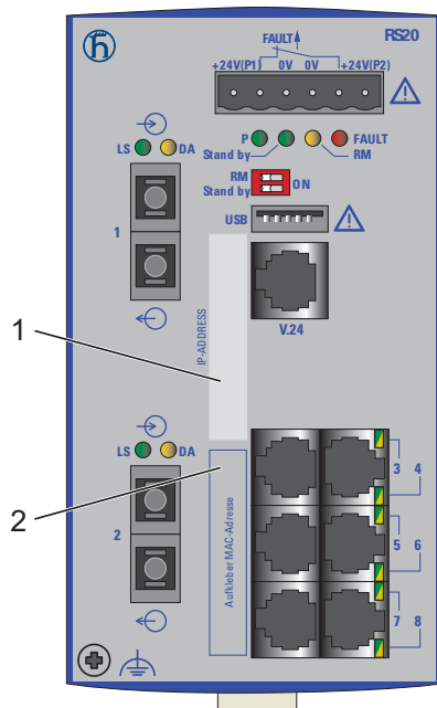
Figure 20: Label area for IP address of device 1 – IP address of device (label area) 2 – MAC address of device (label)
