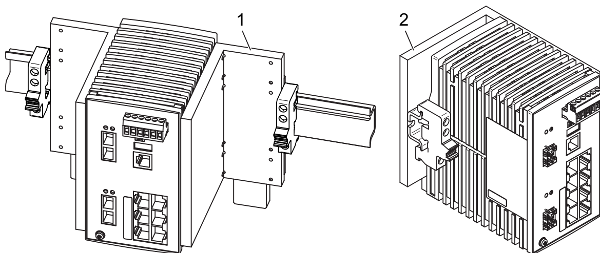
Figure 16: Mounting the RS30-0802... on ships with the Open Rail Mounting Kit 1 - Open Rail Mounting Kit 942 007-001 2 - Open Rail Mounting Kit 942 007-101
