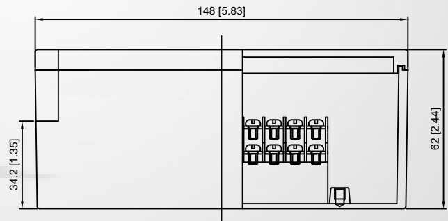
SECTION A - A SHOWN WITH COVER
