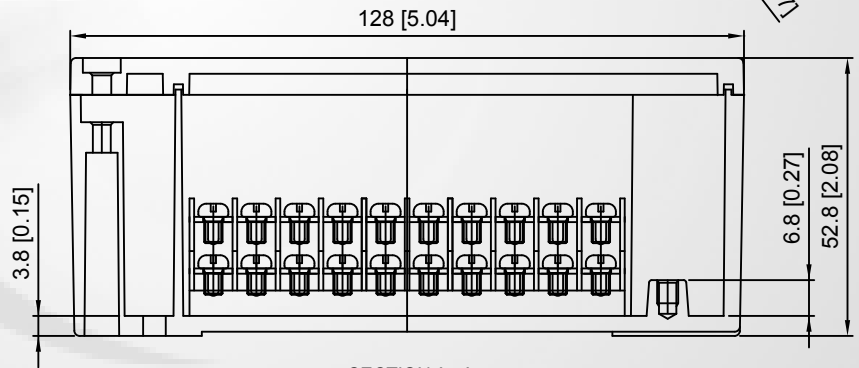
SECTION A - A SHOWN WITH COVER
